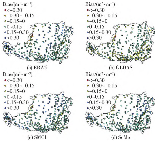
图5 不同产品土壤湿度与站点实测值间偏差空间分布 Fig. 5 Spatial distributions of Bias between soil moisture of different products and site observations on Loess Plateau
