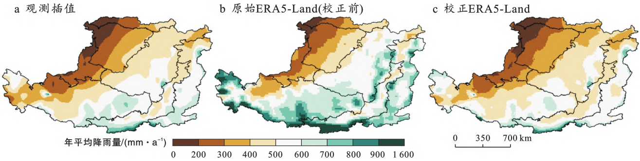
图2 验证期内黄土高原年平均降雨量 Fig.2 Annual average rainfall on Loess Plateau during validation period
