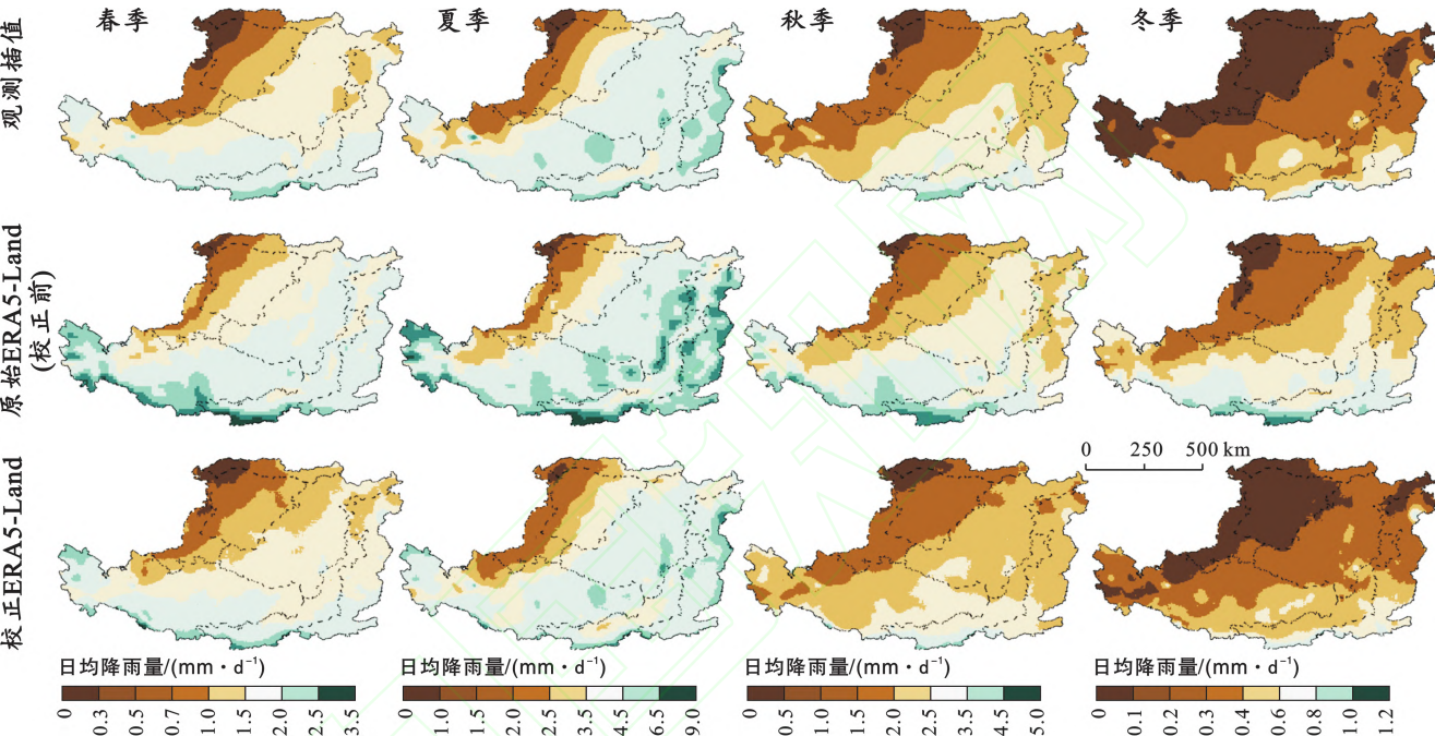
图3 验证期黄土高原的季节性日均降雨量观测插值、ERA5-Land校正前和校正后空间分布 Fig.3 Spatial distribution of seasonal daily average rainfall over Loess Plateau for observed interpolation , ERA5-Land before correction , and ERA5-Land after correction during validation period
