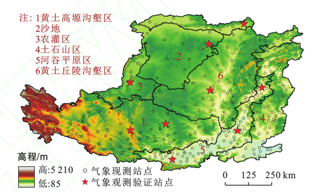
图1 黄土高原研究区及气象站点分布 Fig.1 Loess Plateau study area and distribution of meteorological stations
