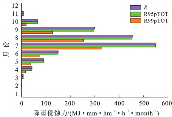
图 6 黄土高原极端降雨的降雨侵蚀力与总降雨侵蚀力的月度对比 Fig.6 Monthly comparison between rainfall erosivity from extreme rainfall and total rainfall erosivity on Loess Plateau
